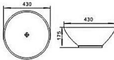
WB-4343R Table Top Basin Size: 430 x 430 x 175 mm RM 250.00
