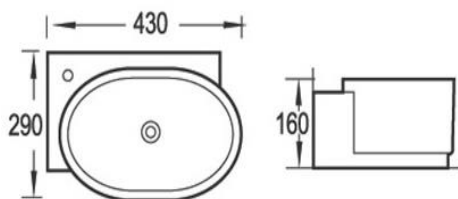
WB-4329R Wall Hung Basin Size: 430 x 290 x 160 mm RM 325.00
