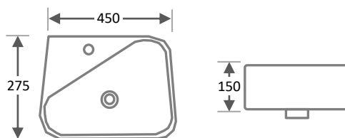
WB-4527 Wall Hung Basin Size: 450 x 275 x 150 mm RM 325.00
