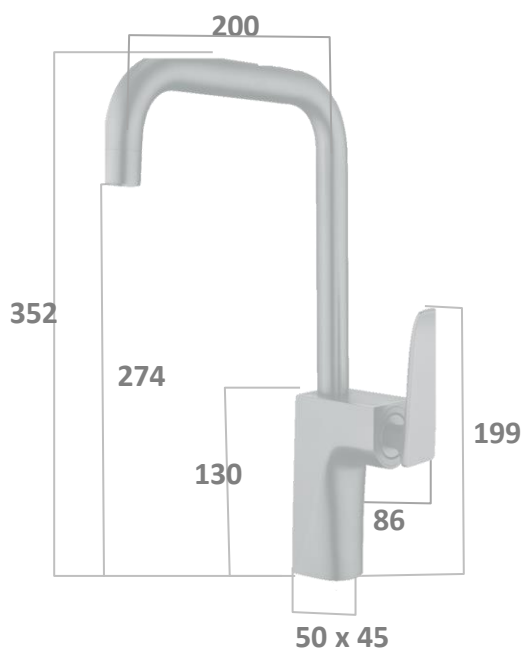
H-KSM-50-472-BL Kitchen Sink Mixer(MATT BLACK)
