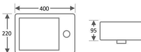
WB-4022 Wall Hung Basin Size: 410 x 220 x 95 mm RM 325.00
