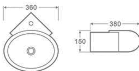
WB-3638C Corner Wall Hung Basin Size: 360 x 380 x 150 mm RM 325.00
