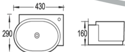
WB-4329L Wall Hung Basin Size: 430 x 290 x 160 mm RM 325.00
